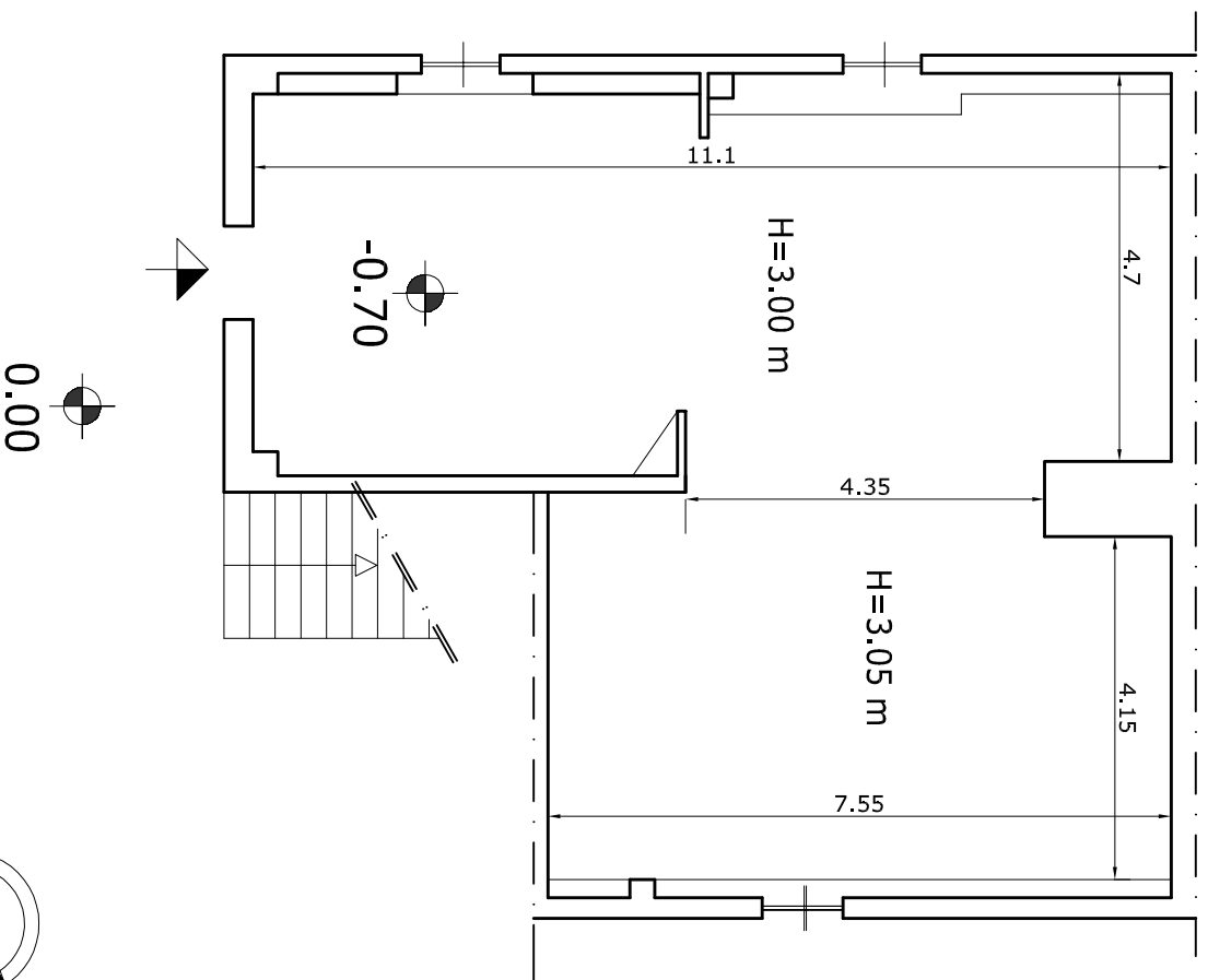
PIANO SEMINTERRATO
